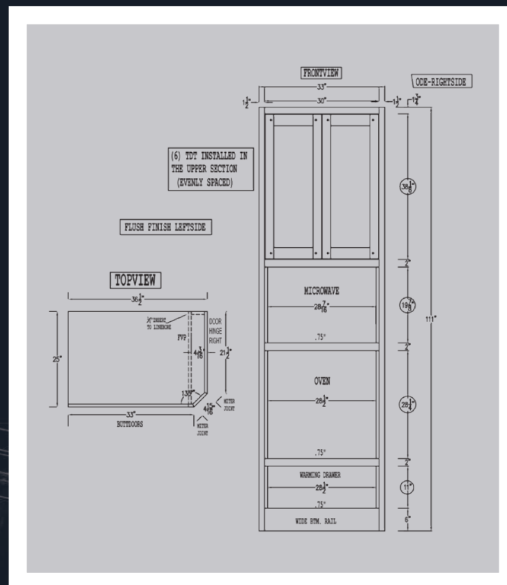
Omega's "Blueprint" Customized Drawing for Quotation
